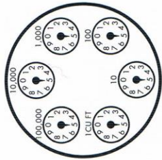
Dial water meter
