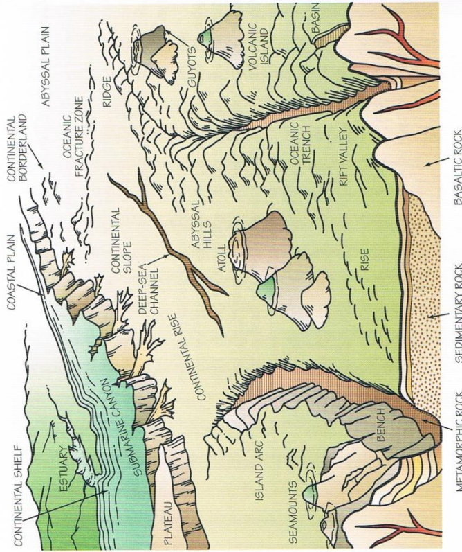
Topographic features of the ocean floor
