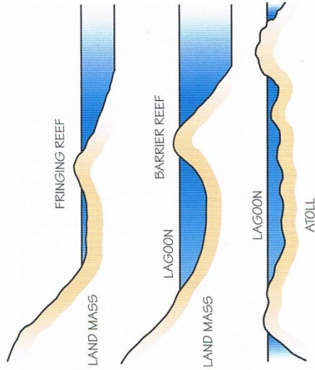
Types of coral reefs
