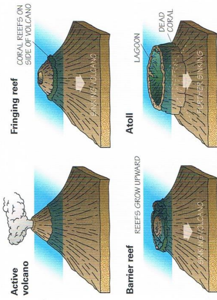
Darwin's theory of the formation of an atoll
