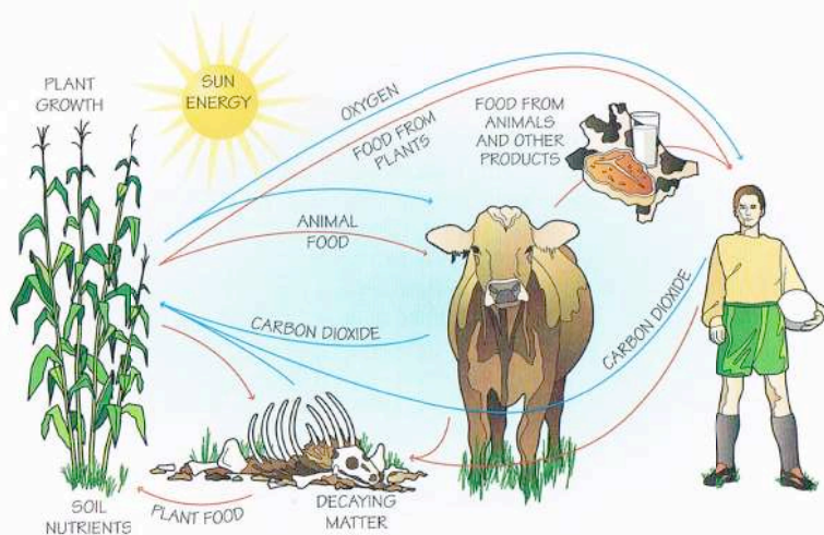
The carbon dioxide–oxygen cycle
