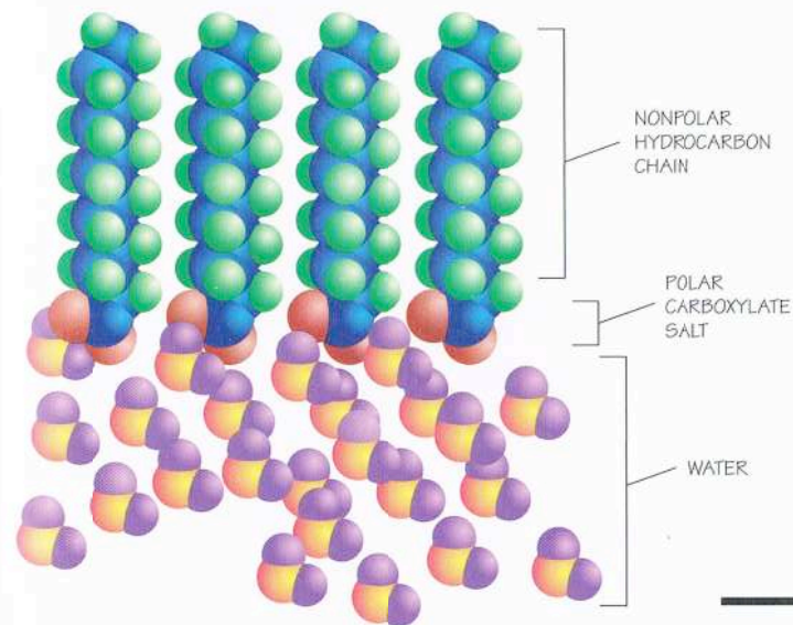
Monolayer of soap on water
