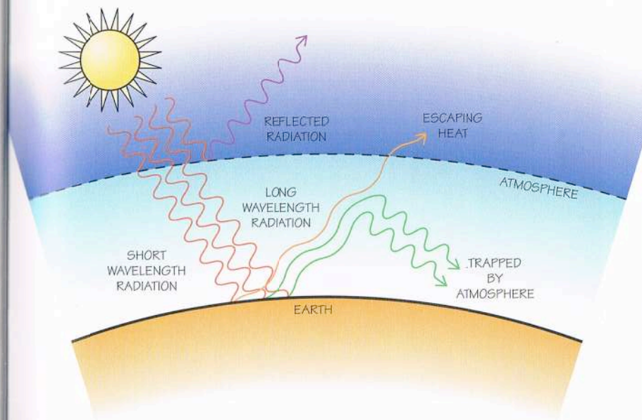
The greenhouse effect
